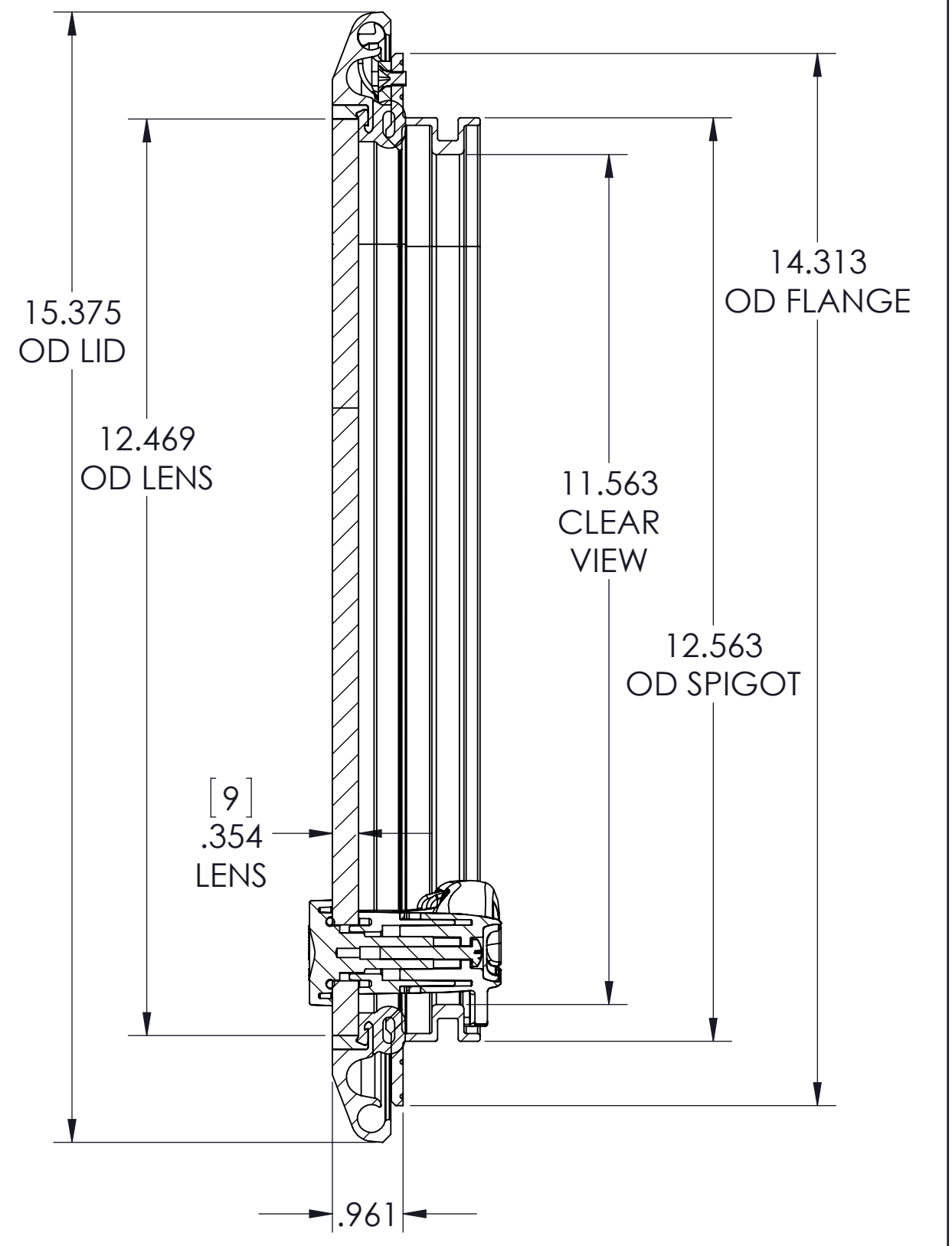
SECTION B-B
